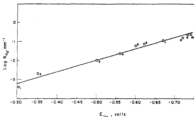
Figure 3. Comparison of oxygen uptake ( \log K_{O_2} ) at -21^\circ\text{C} for \text{Co}(\text{benacen})\text{B} to the polarographic half-wave potentials ( E_{1/2} ) for \text{Co}^{\text{II}}\text{-III}(\text{benacen})\text{B}_2 : 1, \text{PPh}_3 ; 2, \text{CNpy} ; 3, \text{py} ; 4, 3,4-lutidine; 5, piperidine; 6, sec - \text{BuNH}_2 ; 7, 5-Cl- N -MeIm; 8, N -MeIm; 9, i - \text{BuNH}_2 ; 10, n - \text{BuNH}_2 . benacen = benzoylacetylacetonate ion, \text{PPh}_3 = triphenylphosphine, \text{py} = pyridine, and \text{Bu} = butyl (from ref 35).
