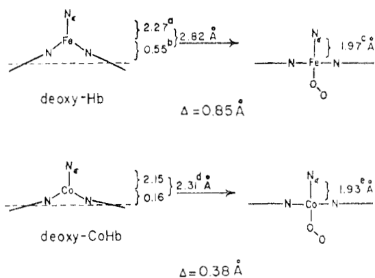
Figure 5. Illustration of the calculation of the total movement of the proximal histidine in Hb (top) and CoHb (bottom). The displacements are taken relative to the 24-atom porphyrin core (from ref 52).
